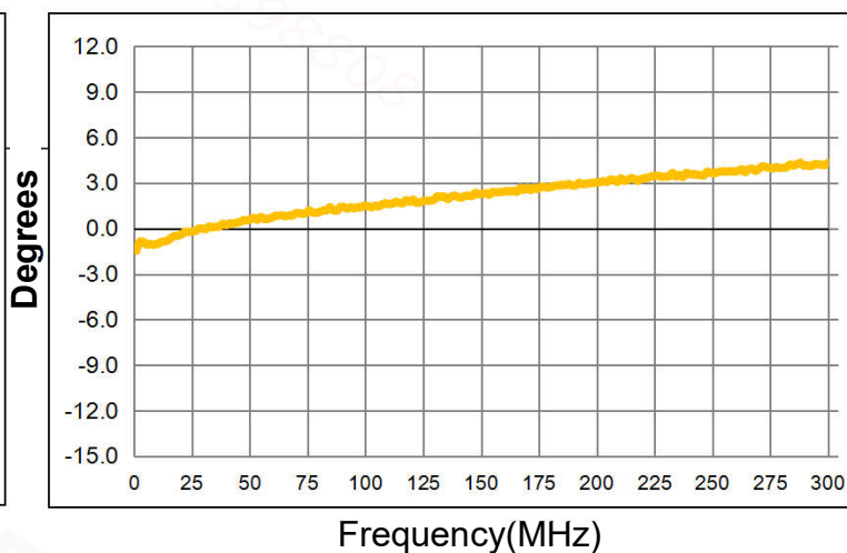
Phase Balance
