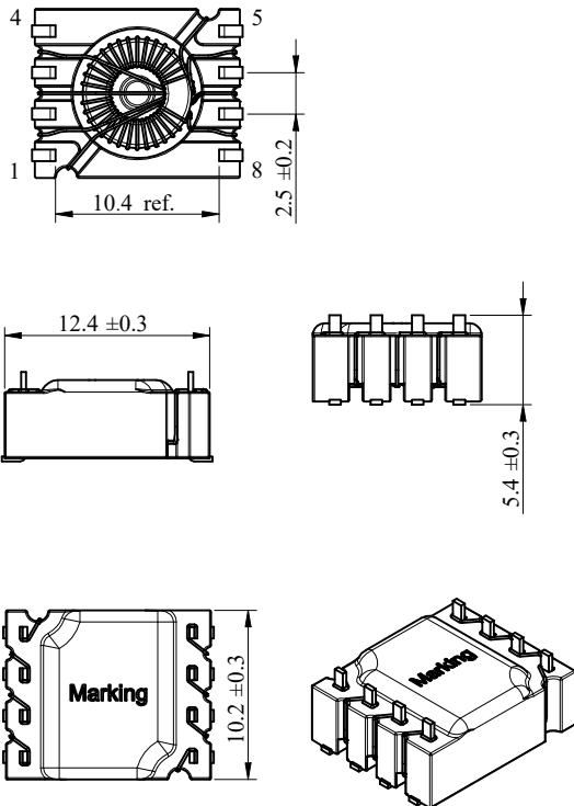
Cosmetic Dimension
