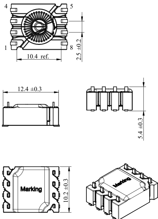
Cosmetic Dimension
