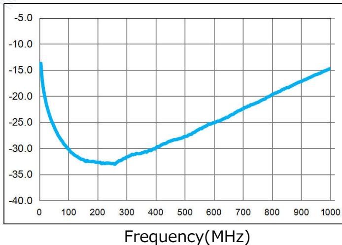
Output 2 Return Loss (Pin6)
